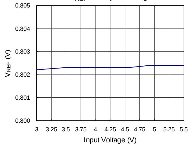
V_{\text{REF}} vs. Input Voltage
